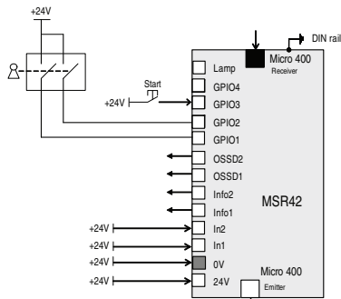
Fixed Blanking, Micro 400 Light Curtain, Manual Reset, No Output Monitoring
