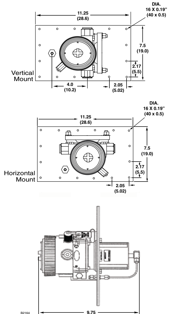
Figure 1—Duct Mount Dimensions in Inches
